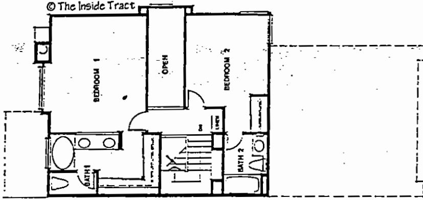
2ND FLOOR
